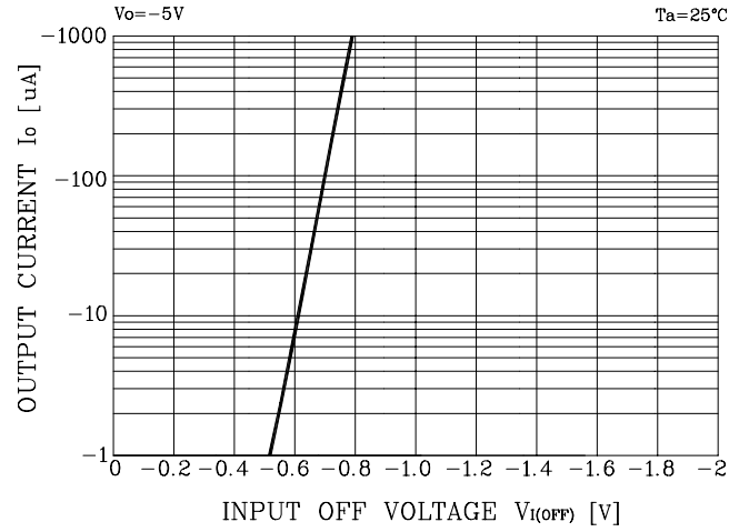
Fig. 2 I_o - V_{I(OFF)}
